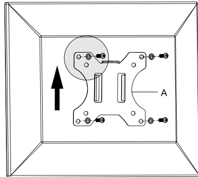
Monitor with a flush installation surface
